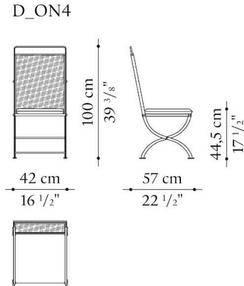
TECHNICAL DRAWING
