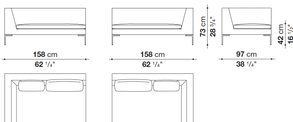
CH156S
