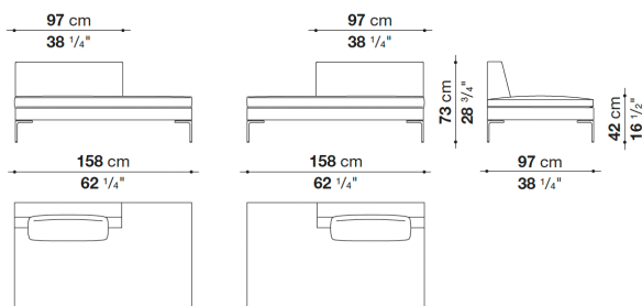
CH156TPS
