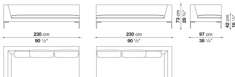
CH228S
