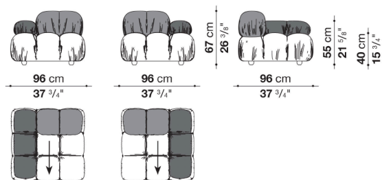
CM96B_TS2 CM96B_TD2
