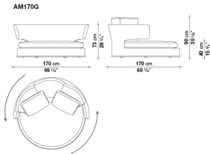
TECHNICAL DRAWING
