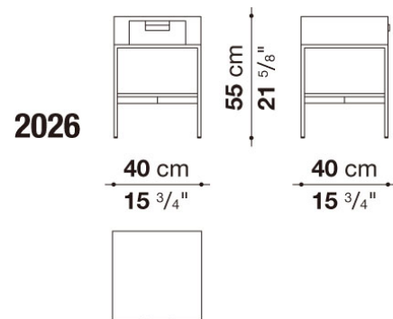
TECHNICAL DRAWING
