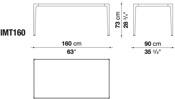
TECHNICAL DRAWING
