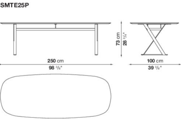
TECHNICAL DRAWING
