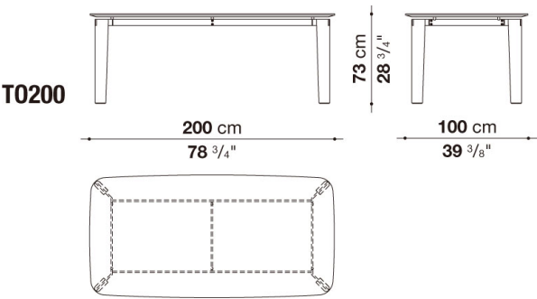
TECHNICAL DRAWING
