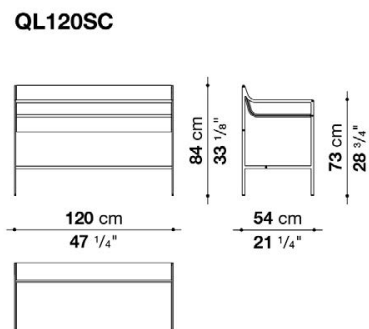
TECHNICAL DRAWING
